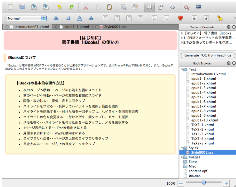
図 1 Book View
